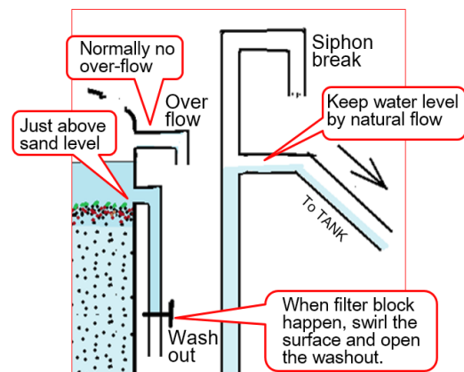
Fig. 17. Height differences of pipes of EPS
