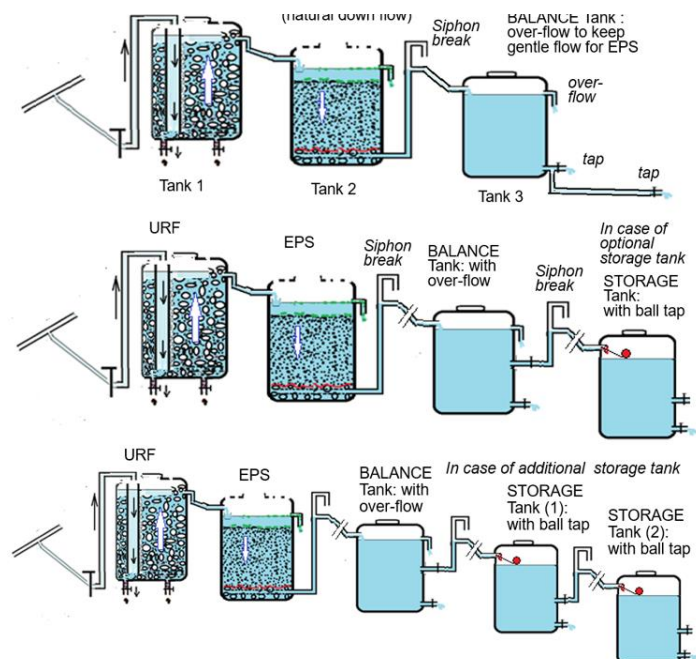
Fig. 32. Addition of public tap and storage tank
