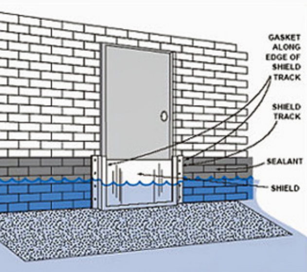
FIGURE 12 (a) Various forms of flood mitigation, (b) Spray on waterproof layer for wall protection
