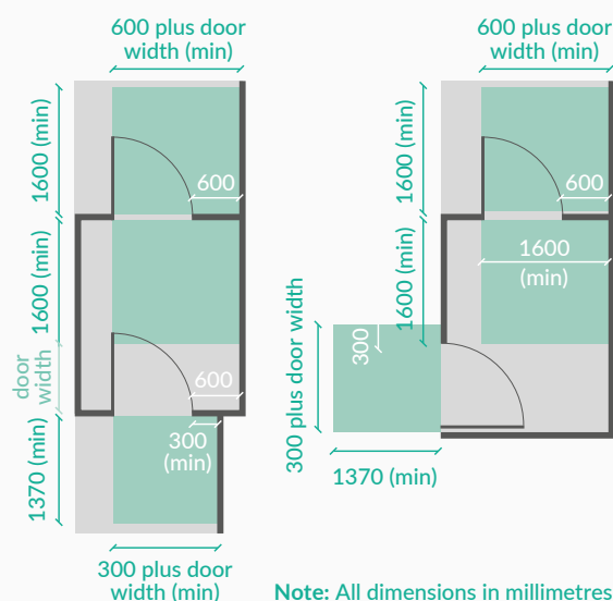
FIGURE 17 Space requirements for building lobbies
