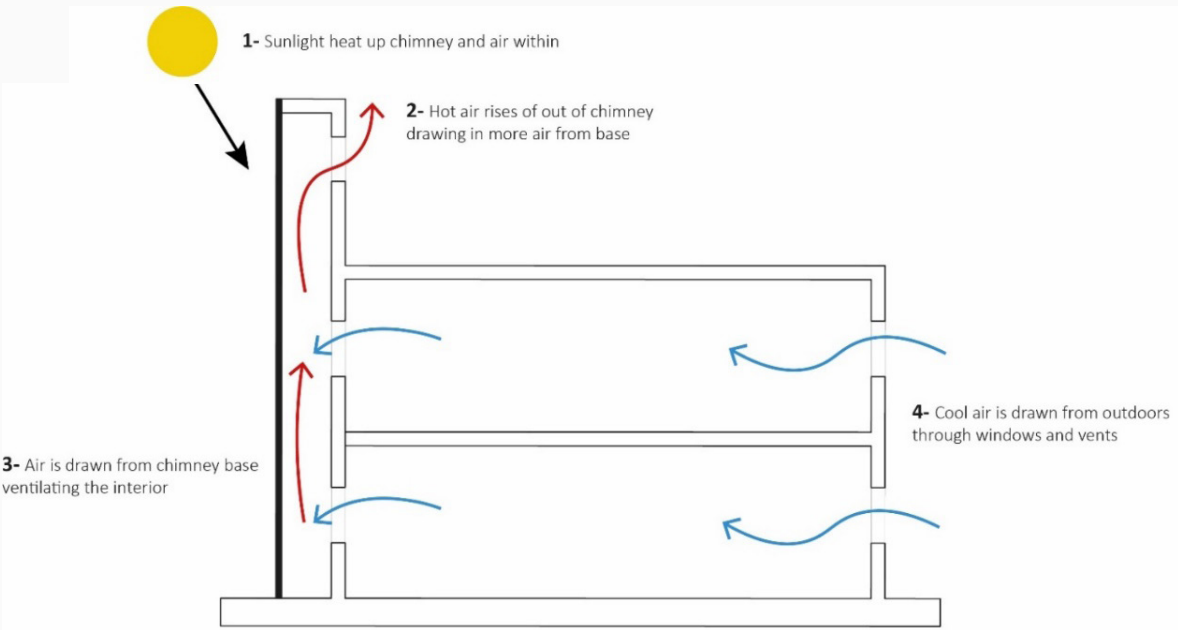
FIGURE 8 Air flow for solar chimneys
